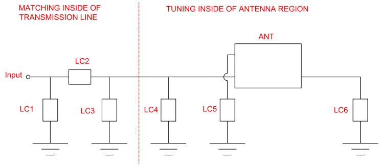
Matching Network Schematic
